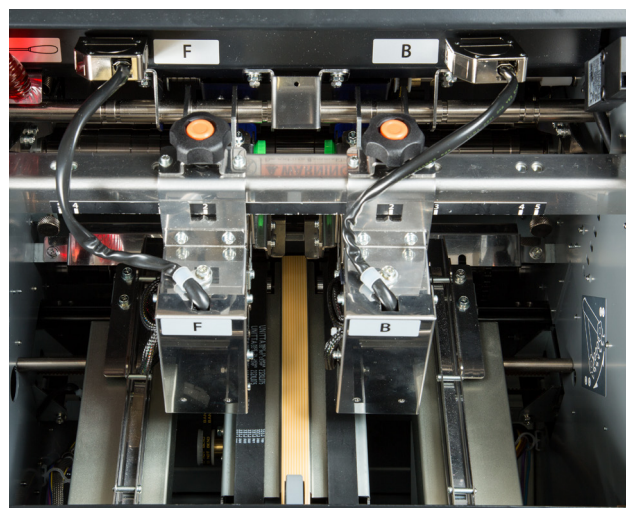
DBM-150 Staple Heads
